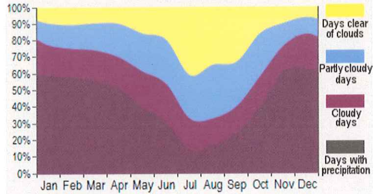
Cloudy Days
