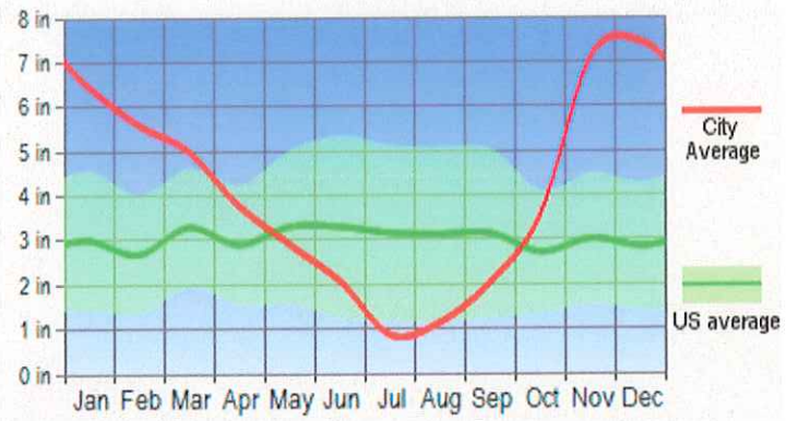
Precipitation
