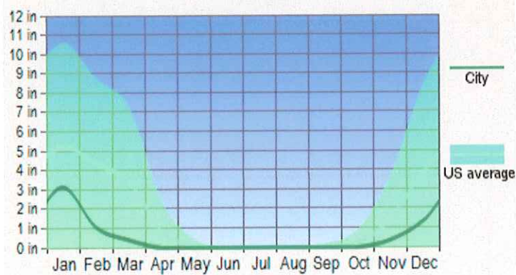
Snowfall
