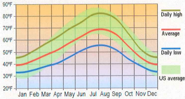
Average Temperatures
