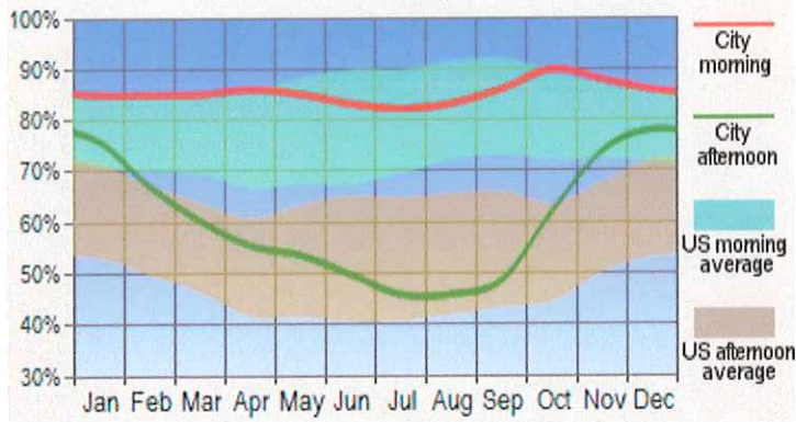
Humidity
